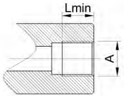
依据锥形英制管螺纹 (BSPT螺纹)
